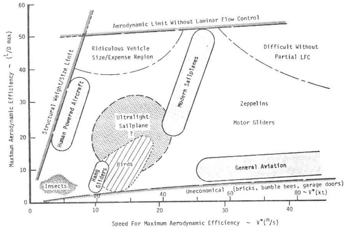
Figure 2: Approximate Boundaries of the Feasible/Economical Low-Speed Flight Spectrum.
