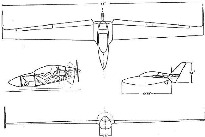
Figure 3: First Place Winner of the SSA/AIAA Student Sailplane Design Competition—Virginia Polytechnic Institute "Callisto".
