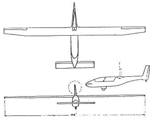
Virginia Polytechnic University "Jake 4011" Two-Place sailplane
