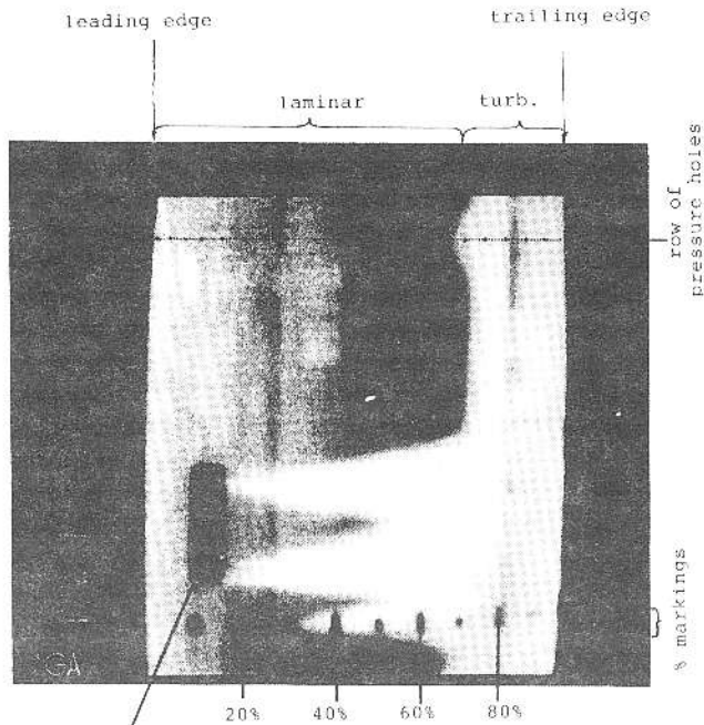
disturbance strip of Aluminium with 0,12 mm height FIGURE 2. Characteristics of an infrared image.
