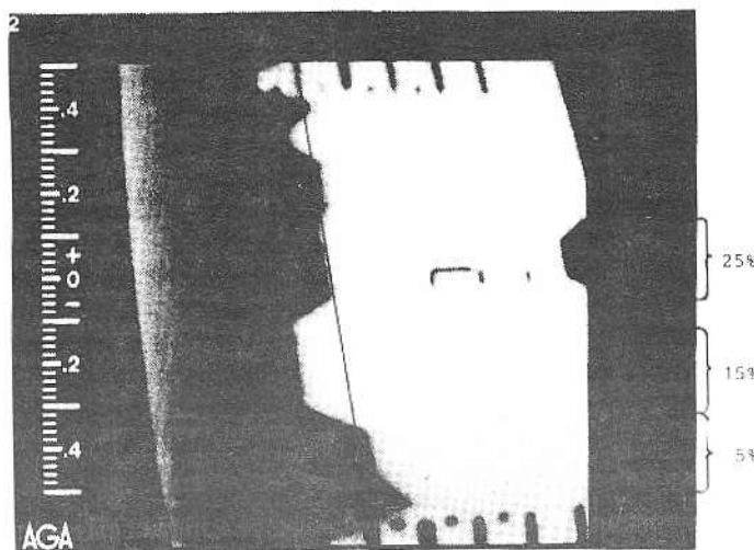
FIGURE 8. Effect of different disturbance positions on transition. LFU glove; \alpha = 0,25^\circ ; \eta_k = 0^\circ ; Re = 9,5 \cdot 10^6 ; disturbance height 0,055 mm; measurement DNW
