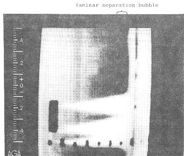
FIGURE 4. Appearance of laminar separation bubble on an infrared image.
