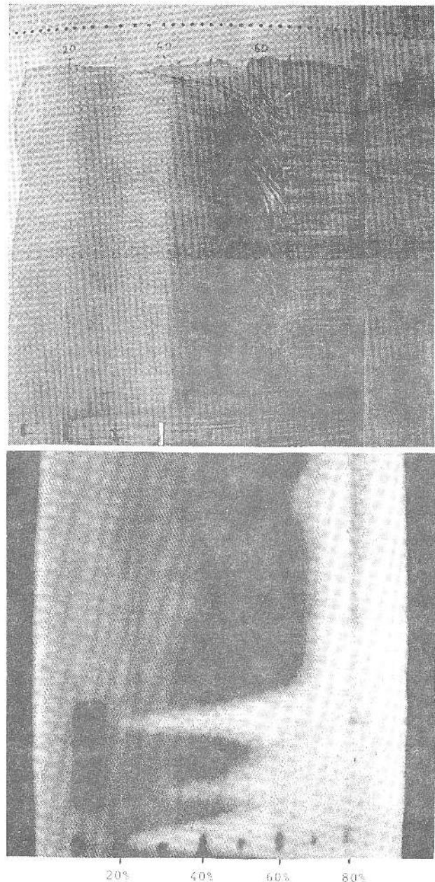
FIGURE 6. Comparison between oil flow picture and infrared image; HQ17/14.38; \alpha = 8^\circ ; \eta_k = 0^\circ ; Re = 1,5 \cdot 10^6 ; meas. MUB
