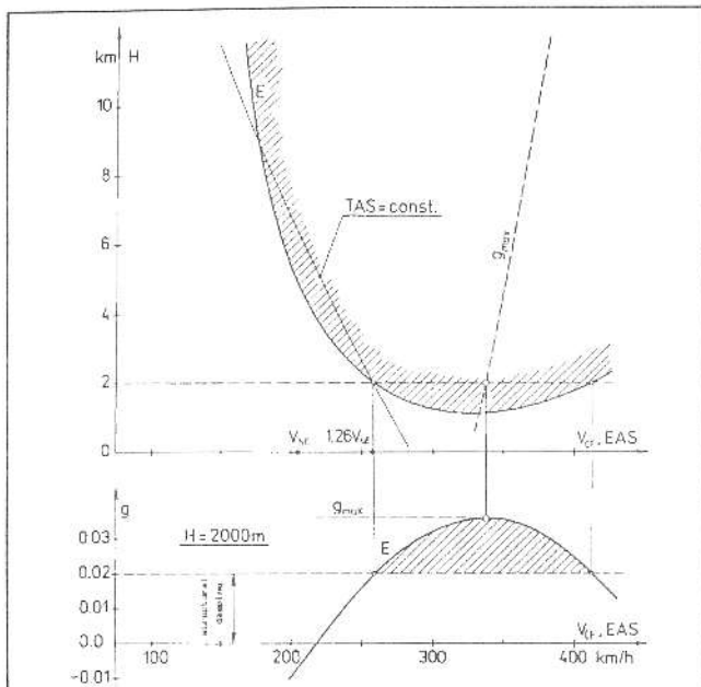
FIGURE 1. Variation of critical speed of symmetrical wing torsion flutter E with rotation and torsion ailerons, with frequency of about 19 Hz. This calculation was made for KR-03A sailplane with reduced torsion ailerons stiffness.
