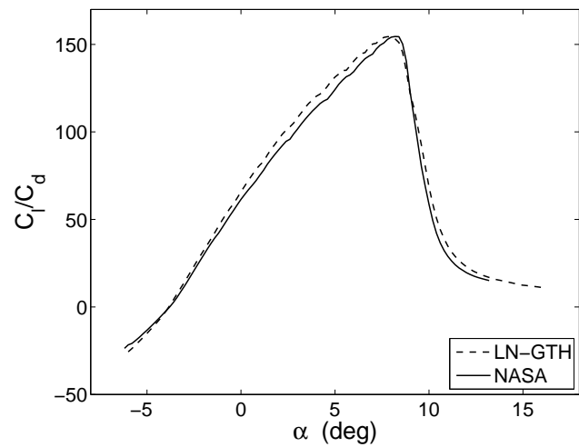
Fig. 12: Performance comparison LN-GTH and NASA airfoil.
