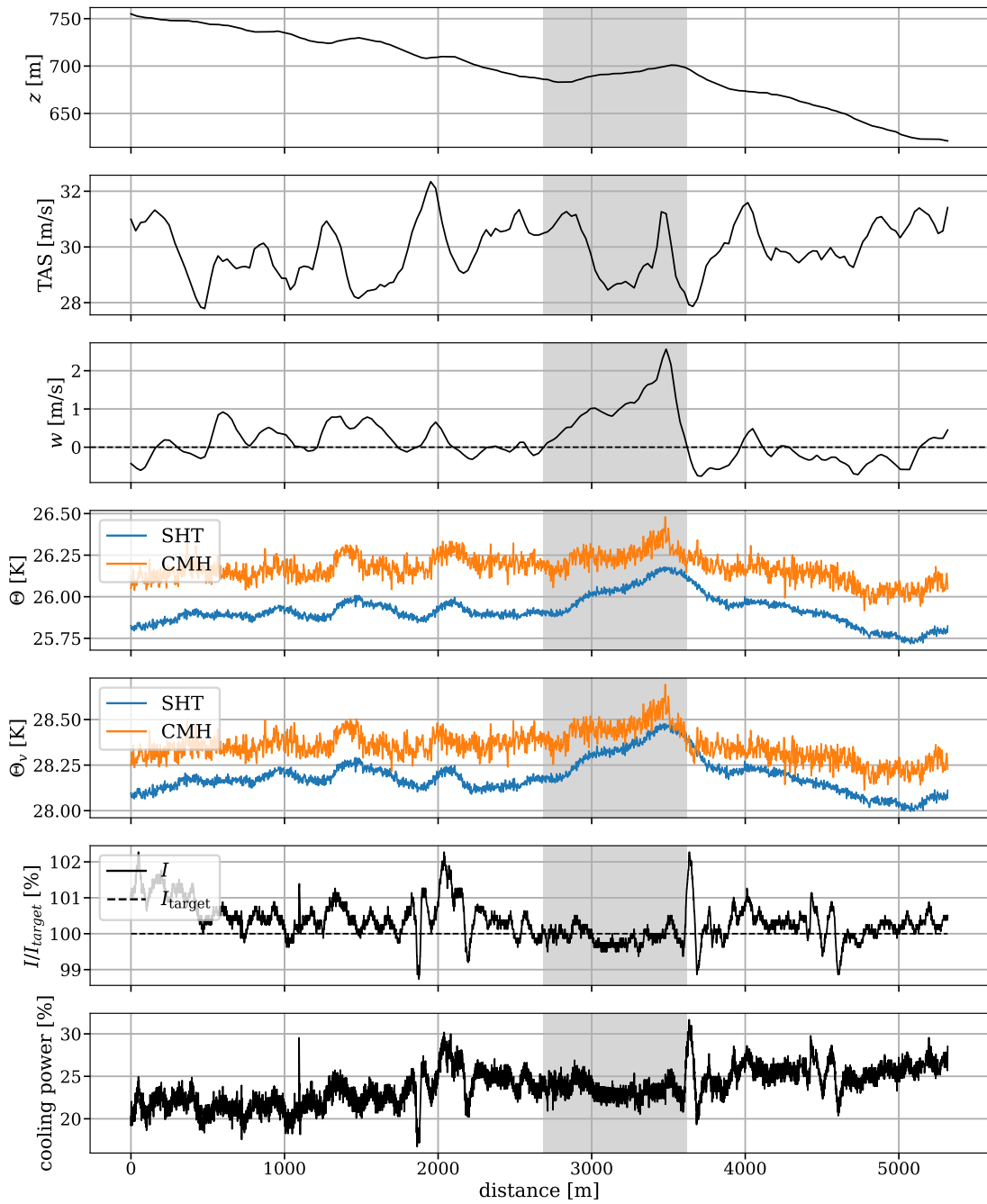
Fig. 6: Representative data log of a straight flight segment containing an headwind thermal pass-through of flight 3. The segment classified as updraft is marked in grey. I/I_{target} represents the measured illuminance relative to the target illuminance, which corresponds to the deviation of the control loop.
