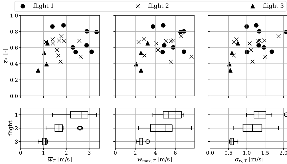
Fig. 8: Mean and maximum updraft velocity, as well as standard deviation of the updraft velocity of the updrafts over the dimensionless height for all measurement sections. The boxplots adhere to the same layout as described in Fig. 7.
