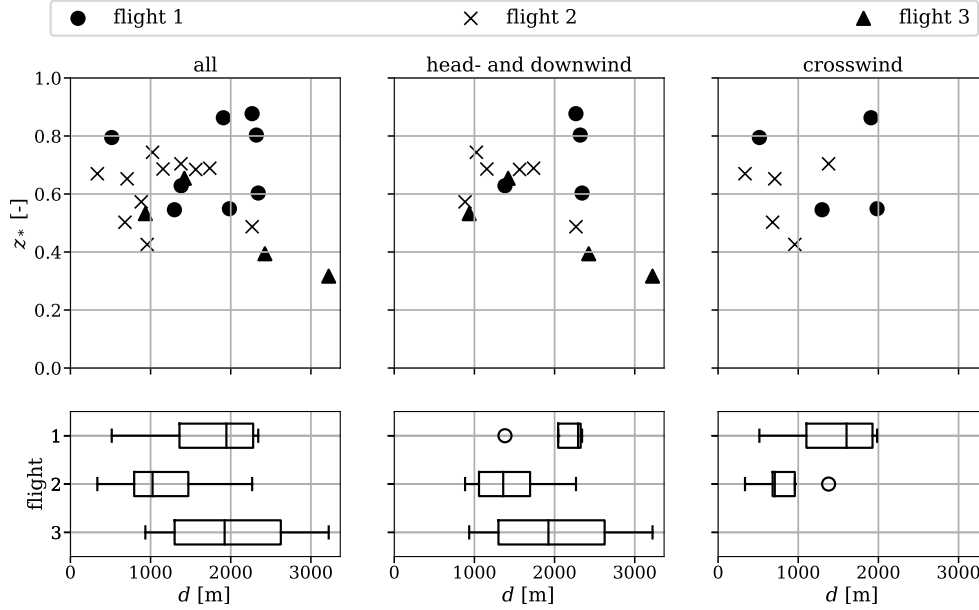
Fig. 7: Horizontal extent of the updrafts above the dimensionless height, for all measurement sections and grouped by measurement sections parallel and perpendicular to the main wind direction. The distribution of the data grouped by flight is shown as boxplots. The boxplots contain the following statistical data: Median: line in box; Interquartile range: box; 1.5 times the interquartile range: “Antennae”; Outliers: points.
