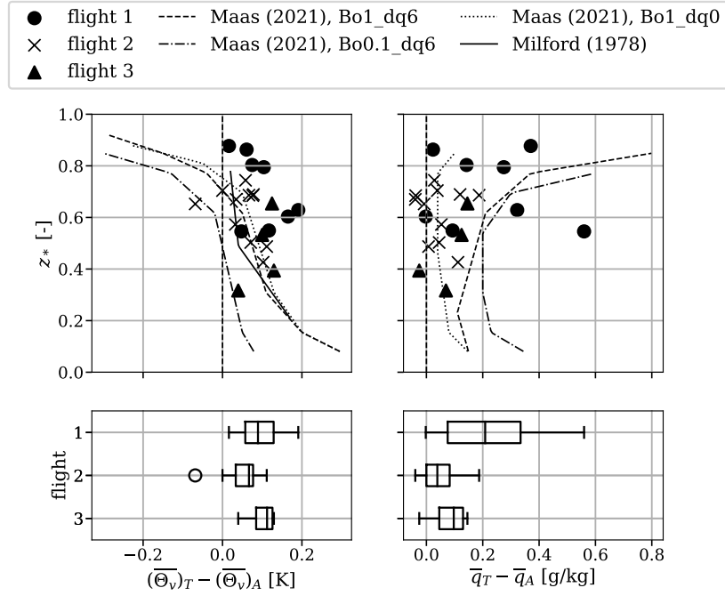
Fig. 9: Difference of the mean virtual potential temperature (measure of density difference, left) and the specific humidity (right) of the updraft to the mean temperature or specific humidity of the measurement section. The lines represent profiles of data available in [26,27]. The boxplot layout is the same as in Fig. 7.
