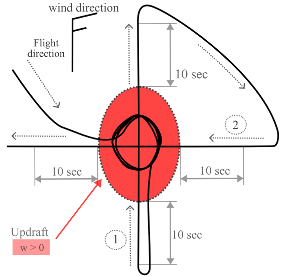
Fig. 5: Flight strategy for measuring thermal cross-section at one altitude (top view of a horizontal slice through the thermal). 1: headwind section, 2: crosswind section.
