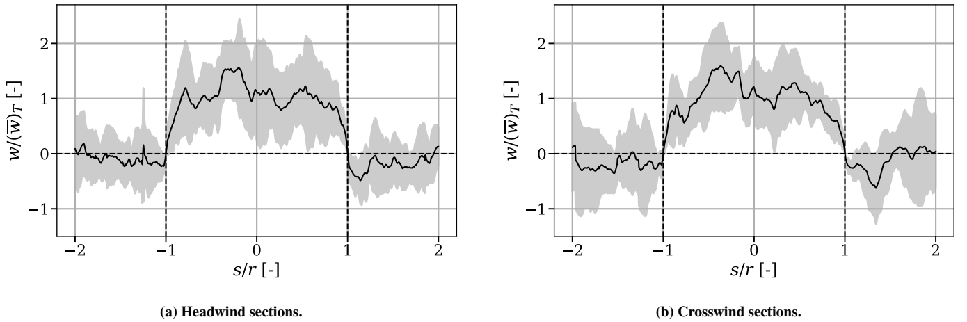
Fig. 10: Averaged courses, or profiles, of updraft velocity over the horizontal normalized distance. The updraft velocity is shown normalized with the mean updraft velocity. The shaded area is the standard deviation of the averaged curve.
