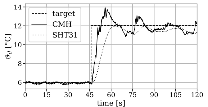
Fig. 2: Response of the sensors to a pseudo-step in the target value of the relative humidity of the climate chamber from 40 % to 60 % at 20 °C (calibrated sensor data). Oscillations around the new target temperature can be attributed to the climate chamber control and water injection system.
