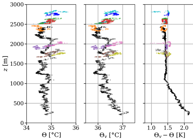
Fig. 4: Measured profiles of the potential temperature and virtual potential temperature of flight 1 (14:34 - 17:21 LT) and the difference between potential and virtual potential temperature to illustrate the contribution of humidity. Only the aerotow and straight measurement sections are shown. The aerotow is shown dotted in black and the measurement sections are color dotted.
