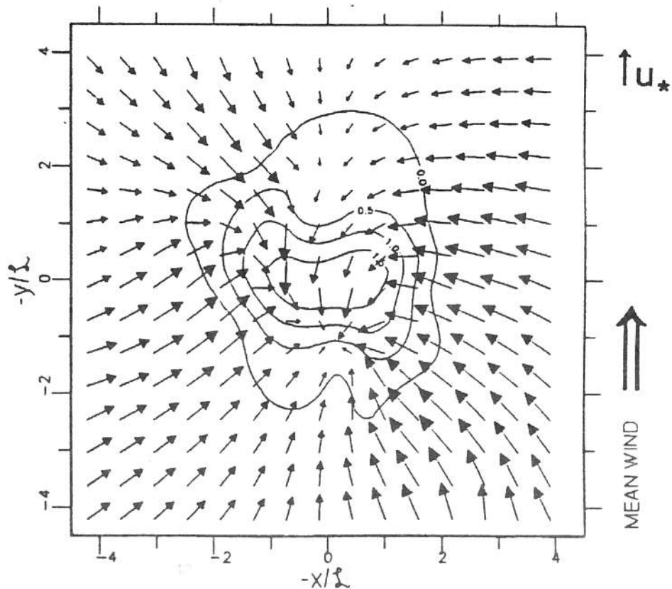
FIGURE 3. As Figure 2, but for -z/L=0.9-1.6 .
