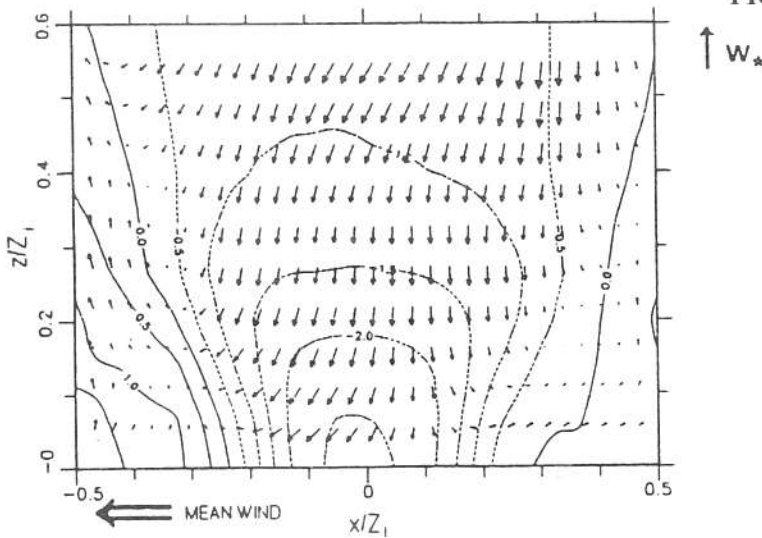
FIGURE 14. As Figure 12, but for "cool-down" event.
