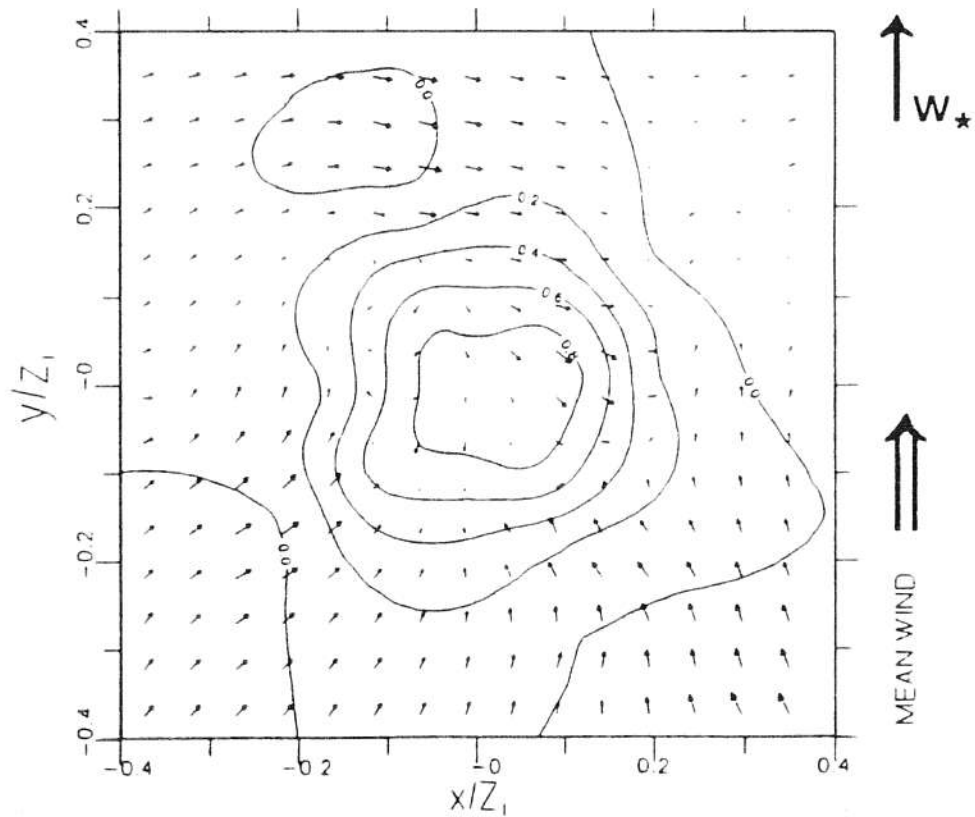
FIGURE 7. As Figure 6, but for 0.3 < z/Z_1 \leq 0.5 .
