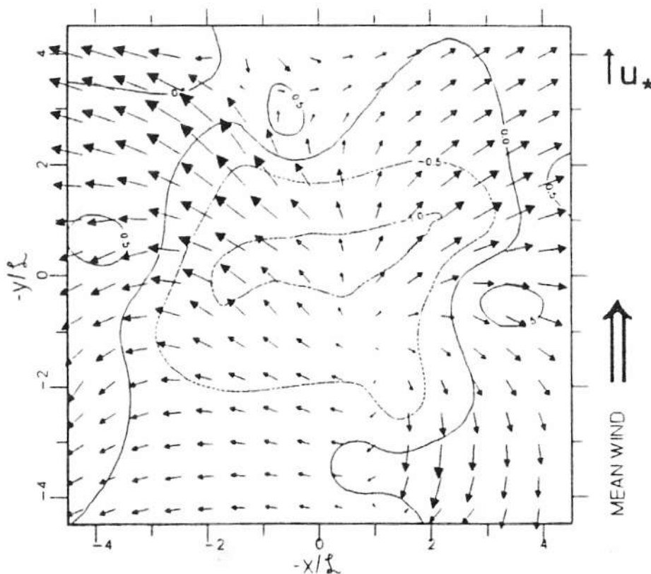
FIGURE 5. As Figure 4, but for -z/L = 0.9 - 1.6 .
