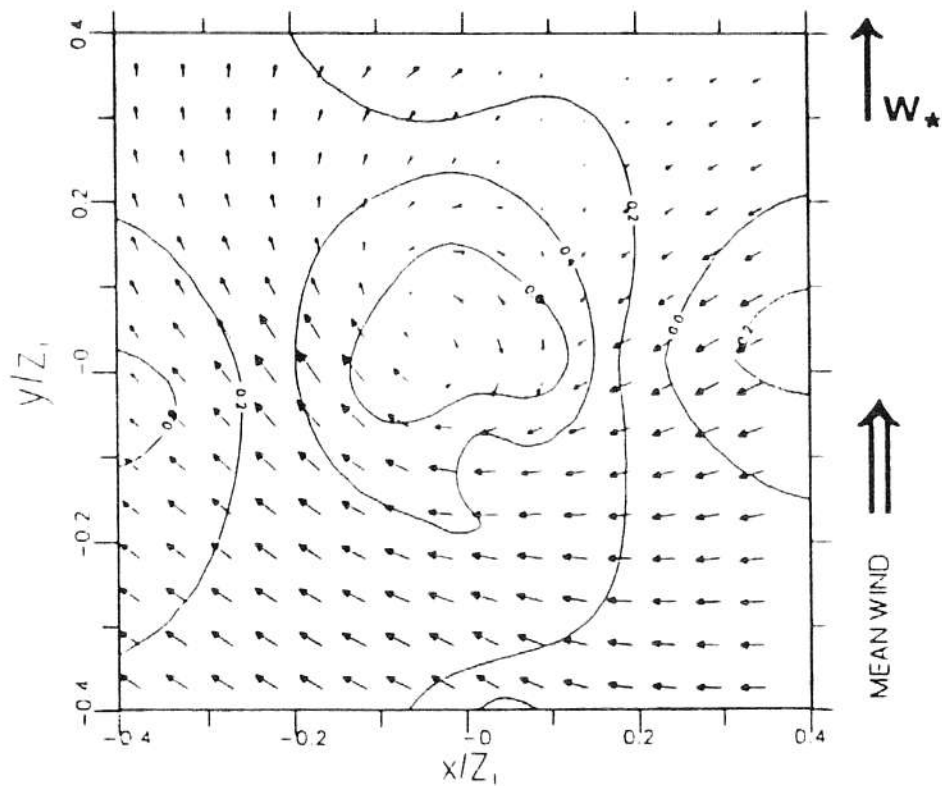
FIGURE 8. As Figure 6, but for 0.5 < z/Z_1 \leq 0.6 .
