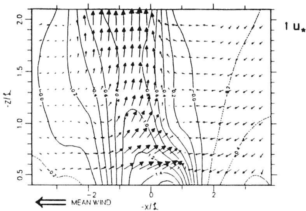
FIGURE 9. Vertical cross-section in the along-wind direction of "warm-up" structure in the SL. Arrows are wind deviations, scaled with u_* . Contours are \theta / \theta_{SL} .
