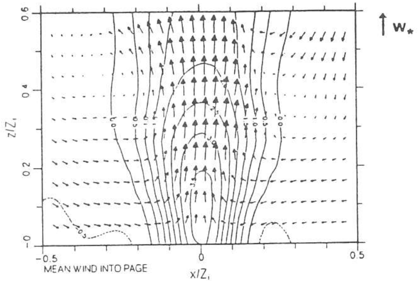
FIGURE 13. As Figure 12, but in the across-wind direction.
