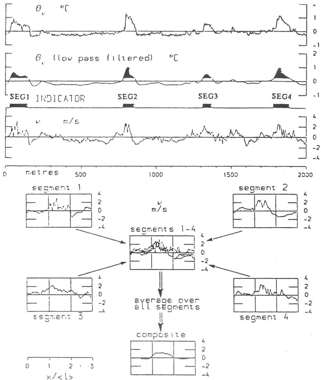
FIGURE 1. A diagrammatic explanation of the compositing method for “warm up” events. For each physical variable, the time series segments corresponding to events defined in the indicator are “cut out” and stretched to a constant number of data points. An equal length on either side of each segment is included in order to represent its immediate environment. Averaging is then performed across corresponding data points of all events, to produce the final composite.
