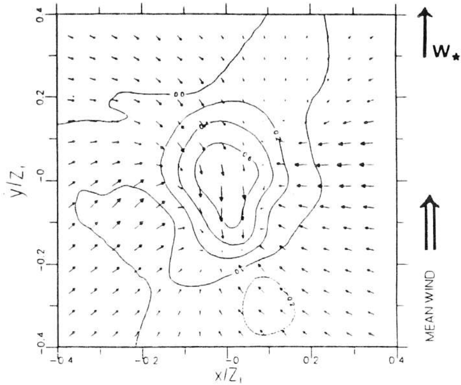
FIGURE 6. Horizontal cross-section of "warm up" structure in the ML for the height range 0.15 < z/Z_1 \leq 0.20 . Arrows are horizontal wind deviations, scaled with w_* . Contours are w/w_* .
