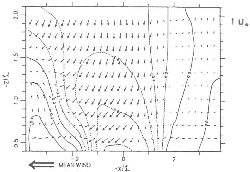
FIGURE 11. As Figure 9, but for "cool-down" structure.
