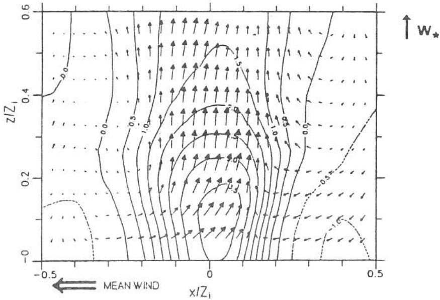
FIGURE 12. Mixed layer "warm-up" vertical cross-section in the along-wind direction. Arrows are wind deviations, scaled with w_* . Contours are \theta / \theta_* .
