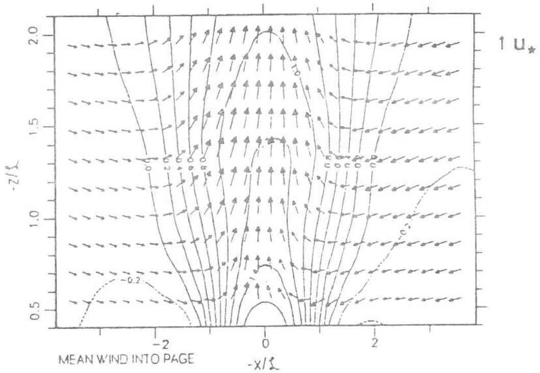
FIGURE 10. Vertical cross-section in the across-wind direction of "warm-up" structure in the SL. Arrows are wind deviations, scaled with u_* . Contours are \theta/\theta_{SL} .
