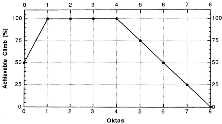
Figure 4 Reduction of achievable lift rates by convective cloud cover.
