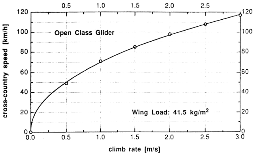
Figure 1 Cross-country flight speed vs. climb rate for an open class sailplane.
