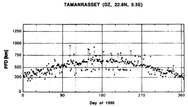
Figure 7 Potential flight distances for Tamanrasset (DZ) in 1996.
