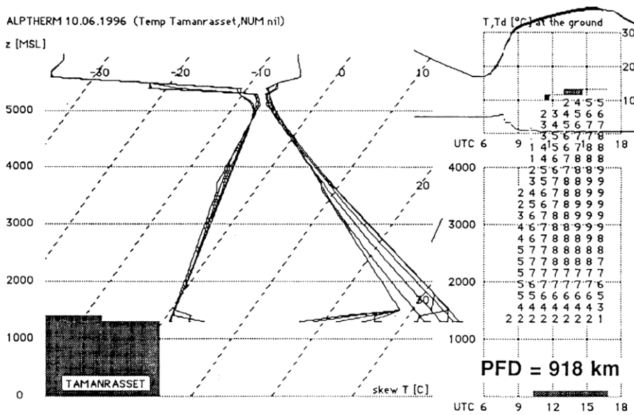
Figure 2 Simulation of convection by ALPTHERM. Evolution of the thermodynamic profiles (left), time-altitude cross-section of lift-rates and convective cloud cover (lower right), evolution of ground values (upper right).
