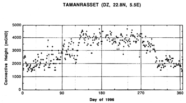
Figure 8 Height of convection at Tamanrasset (DZ) in 1996.
