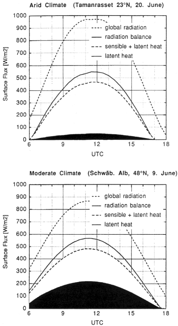
Figure 6 Surface fluxes in ALPTHERM for arid (top) and moderate (bottom) climates.
