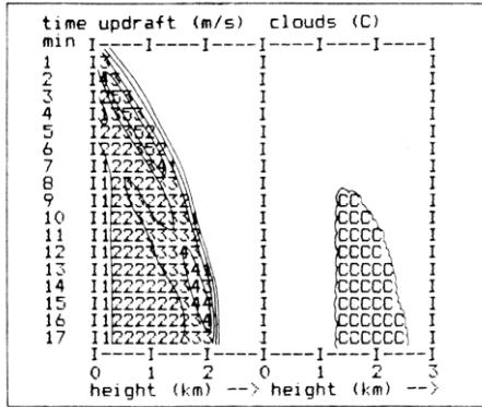
Figure 2 Simulation of thermal updraft and cumulus clouds on the base of the predicted profiles for 13 CEST.
