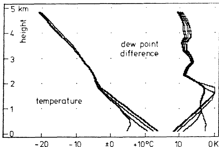
Figure 1 Predicted vertical profiles of temperature and dewpoint difference for "Westliches Münsterland" on May 28, 1983.
