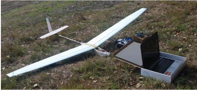
Figure 6 The UAV system, including the ground station.
