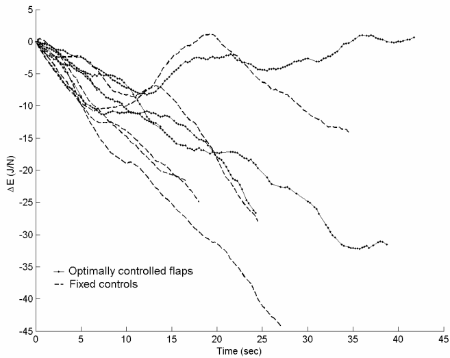
Figure 8 Flight test 1: Variation of specific total energy.
