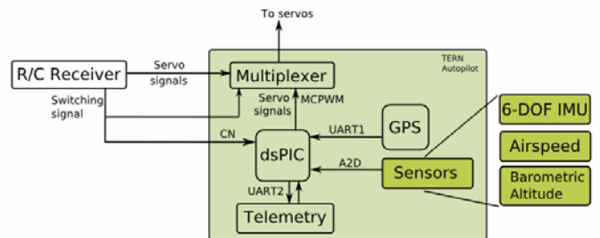
Figure 5 Block diagram of autopilot components.
