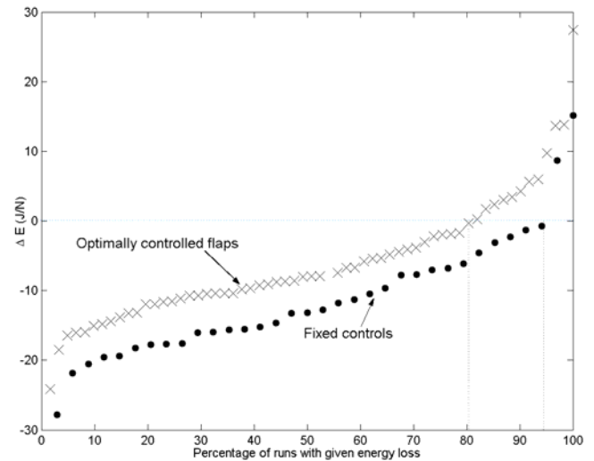
Figure 10 Effect of active control of flaps on energy loss.
