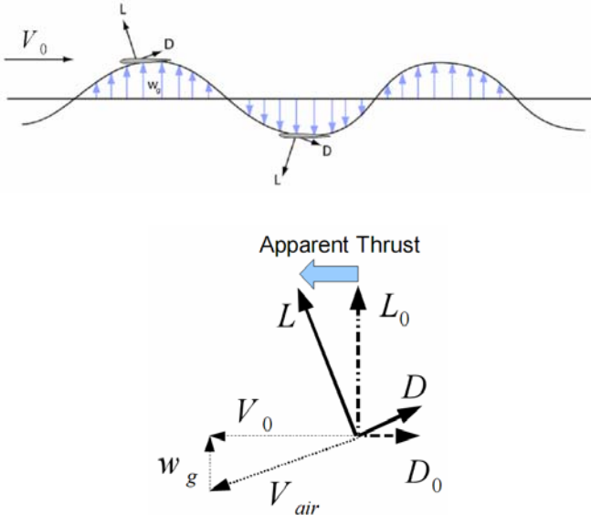
Figure 1 The fundamental concept of gust soaring.
