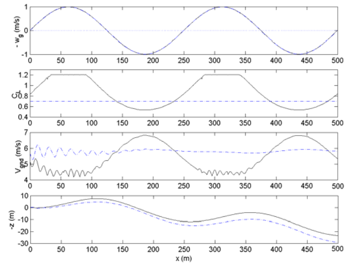
Figure 4 Optimized control law simulated over a sinusoidal gust with \lambda = 250 m.
