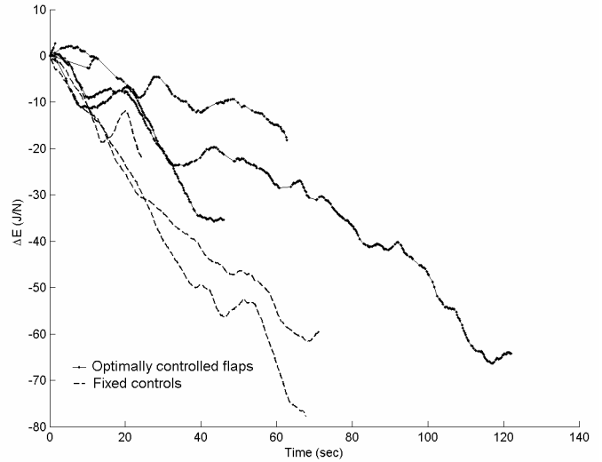
Figure 9 Flight test 2: Variation of specific total energy.
