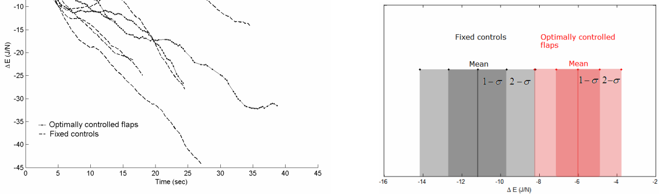
Figure 8 Flight test 1: Variation of specific total energy.
